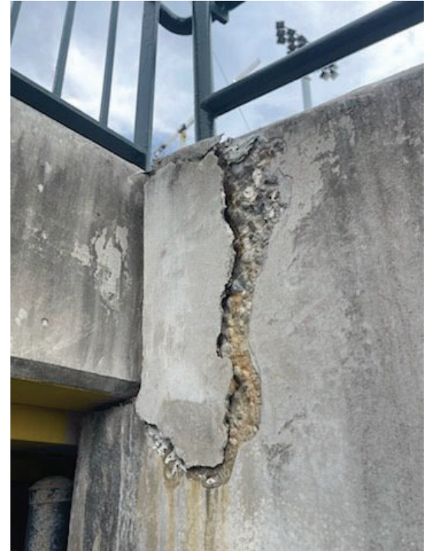
Miscellaneous concrete repairs throughout stadium to eliminate failures and trip hazards
