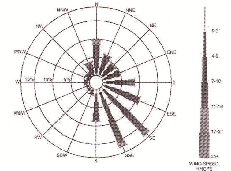
Figure 1 Wind Rose for Corpus Christi, TX
