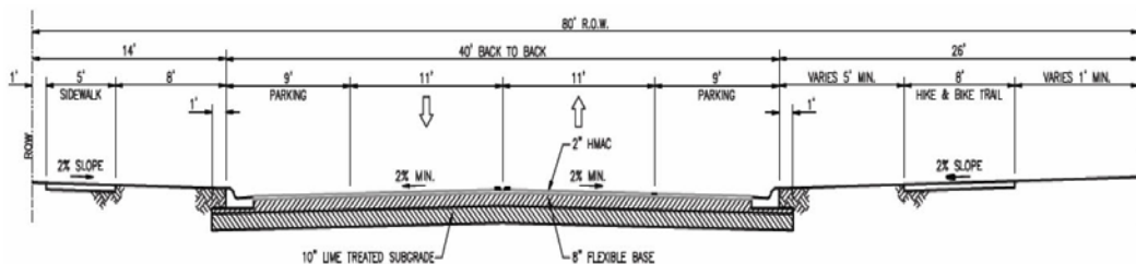
P1 Street Section
