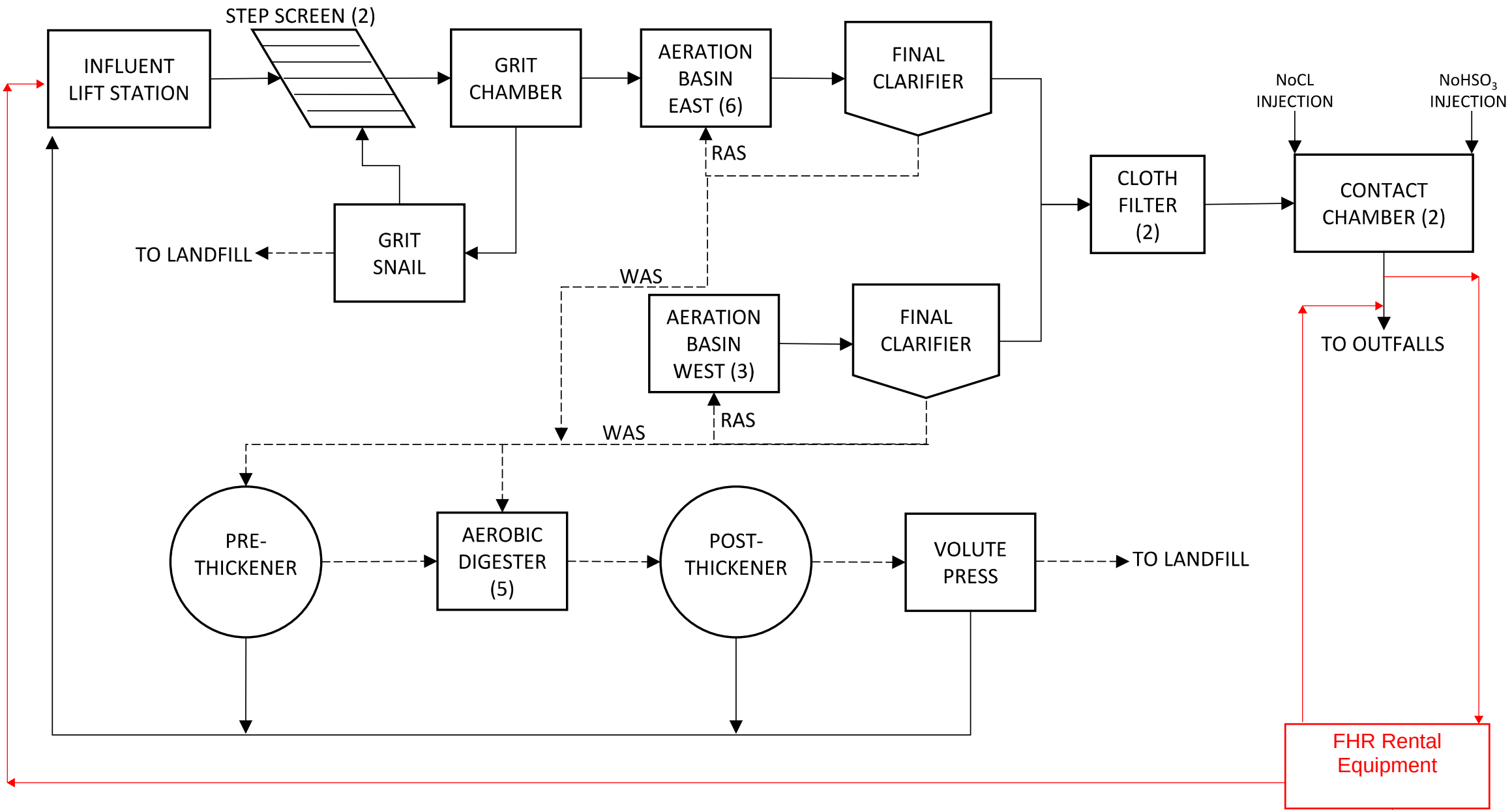
ALLISON WASTEWATER TREATMENT FACILITY TPDES PERMIT RENEWAL APPLICATION PROCESS FLOW DIAGRAM
