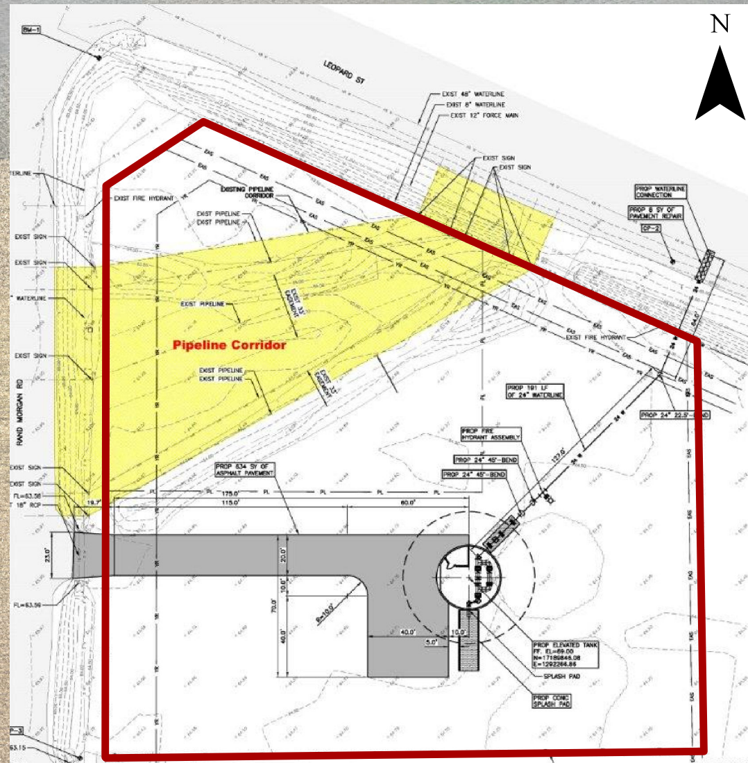
Rand Morgan Elevated Storage Tank Site Plan
