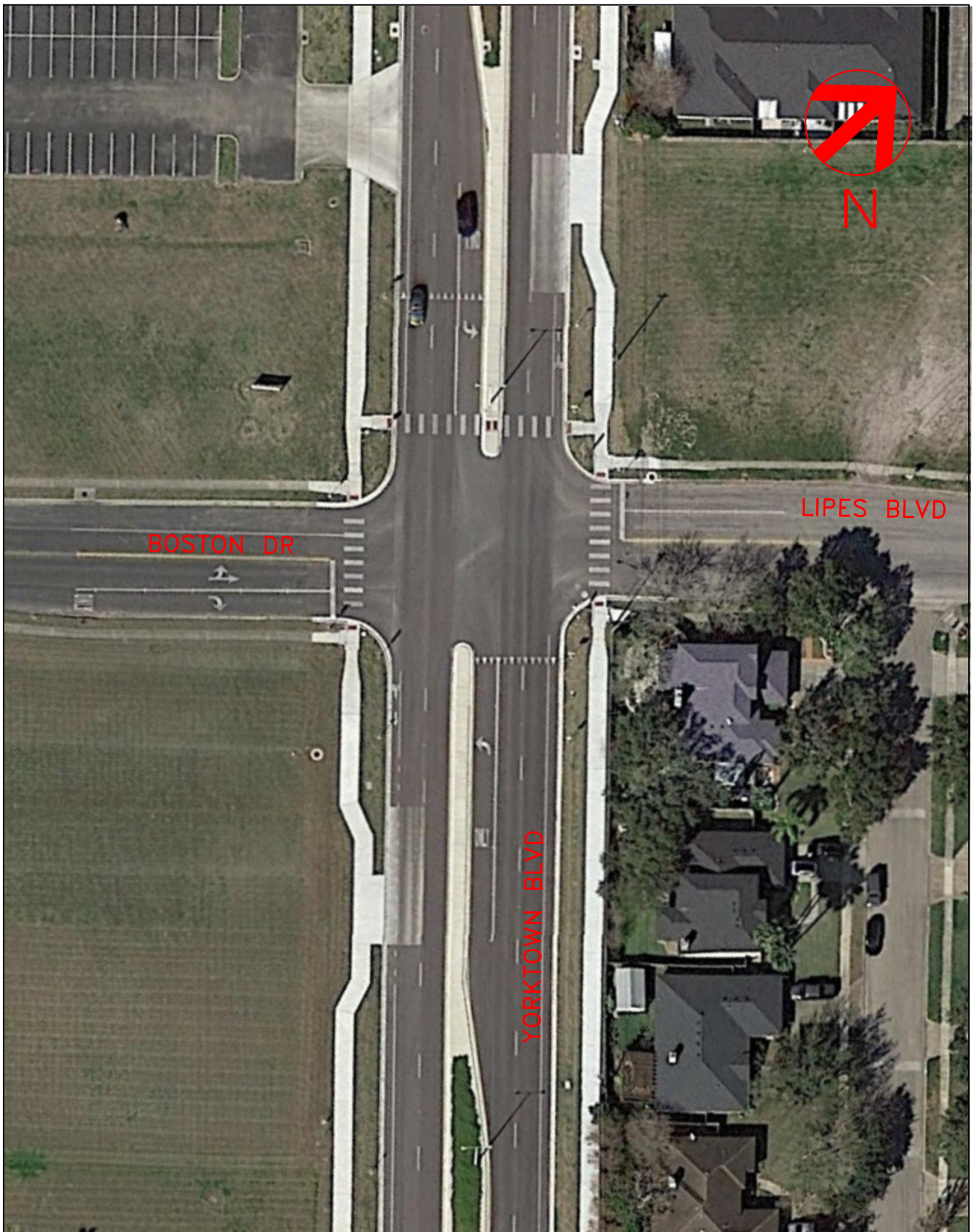
EXHIBIT PEDESTRIAN CROSSING IMPROVEMENTS ON YORKTOWN BLVD AND LIPES BLVD/BOSTON DR
