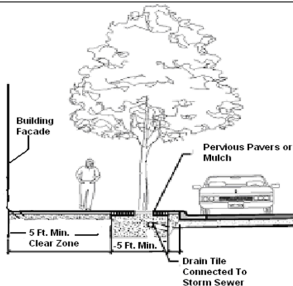
Figure 6.13.2.I.2. Tree Trench and Tree Pit Section
